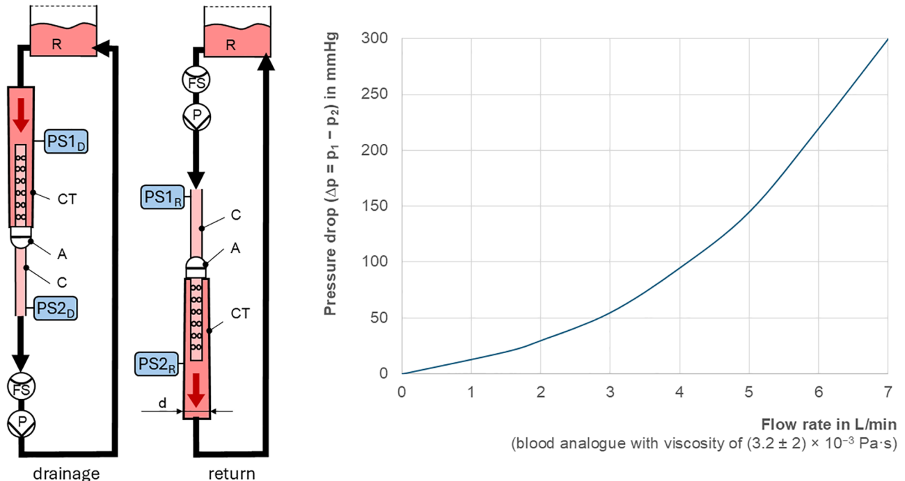
Figure 2. Testing ECLS cannula. Left: Example of test circuit for pressure drop measurement in drainage and return cannula. Right: Graph with exemplary test results. A, access port with seal; C, cannula under test; CT, cylindrical test chamber with d = 2 \times diameter of cannula under test; FS, flow sensor; P, pump; PS1 D and PS2 D , pressure sensors 1 and 2 for drainage cannula; PS1 R and PS2 R , pressure sensors 1 and 2 for return cannula; R, reservoir for blood analog.
