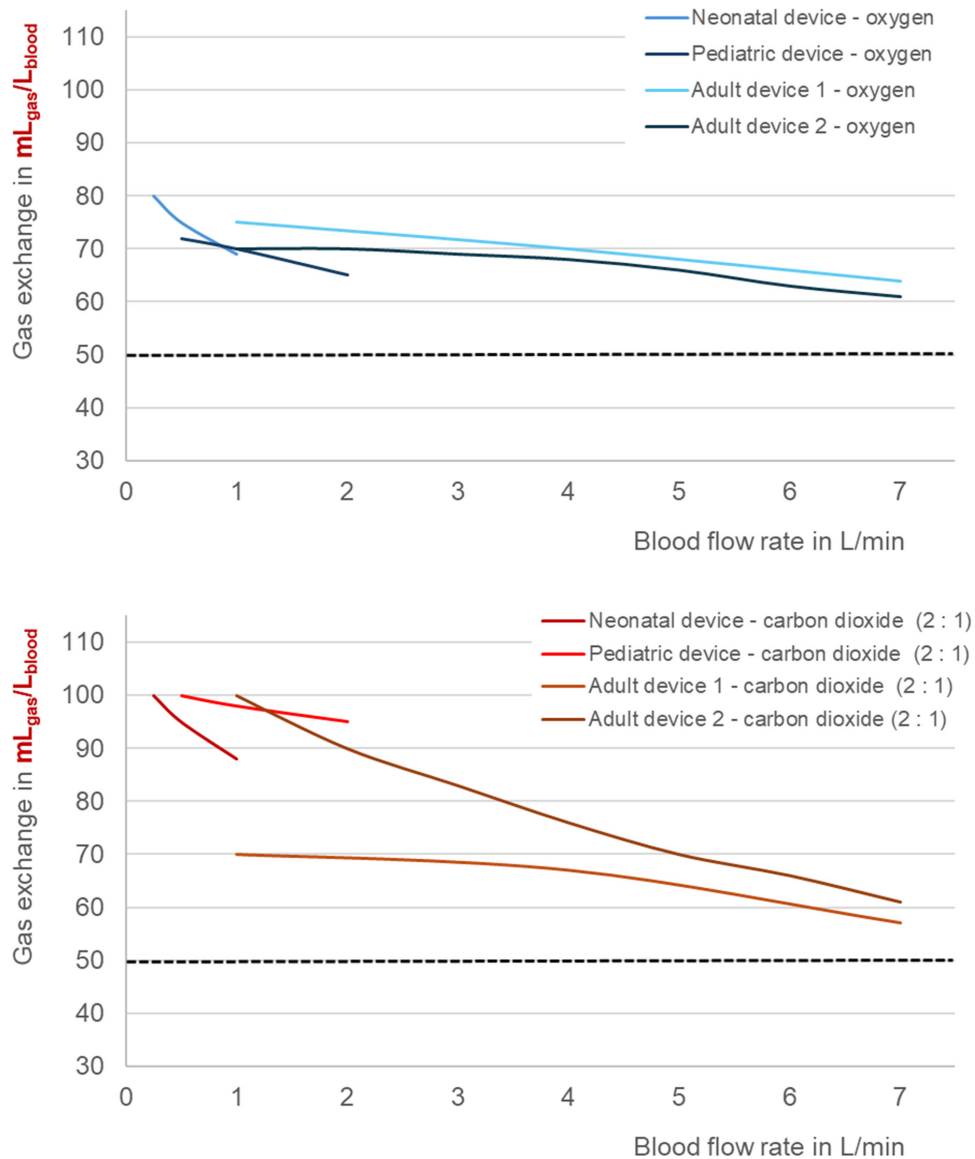
Figure 5. Exemplary depiction of gas exchange (in \text{mL}_{\text{gas}}/\text{L}_{\text{blood}} ) over a range of blood flow rates for oxygen (top graph) and carbon dioxide (bottom graph; at a gas-to-blood flow ration of 2: 1). The lower limit of 50 \text{ mL}_{\text{gas}}/\text{L}_{\text{blood}} for oxygen exchange (and for carbon dioxide exchange at a respiratory quotient of 1) is marked as dashed horizontal line.
