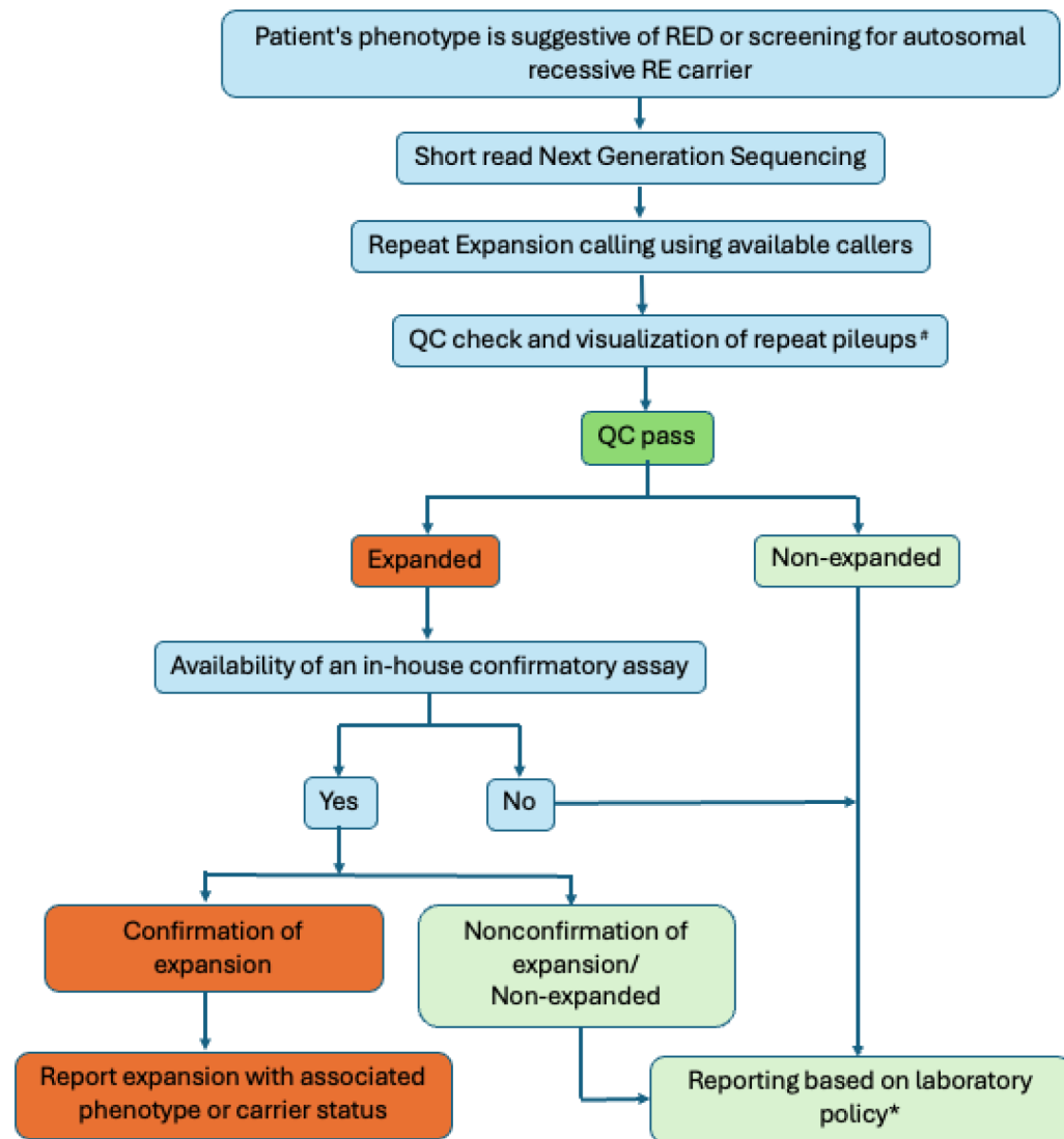
Figure 1. Laboratory flow chart for confirmation and reporting of RE loci using short-read NGS. #QC performance metrics developed during the clinical validation studies. Low-quality calls are due to ambiguous read mapping or insufficient read support. *In the absence of an in-house confirmatory assay, QC passed expansion could be reported with an appropriate recommendation for follow-up confirmation.
